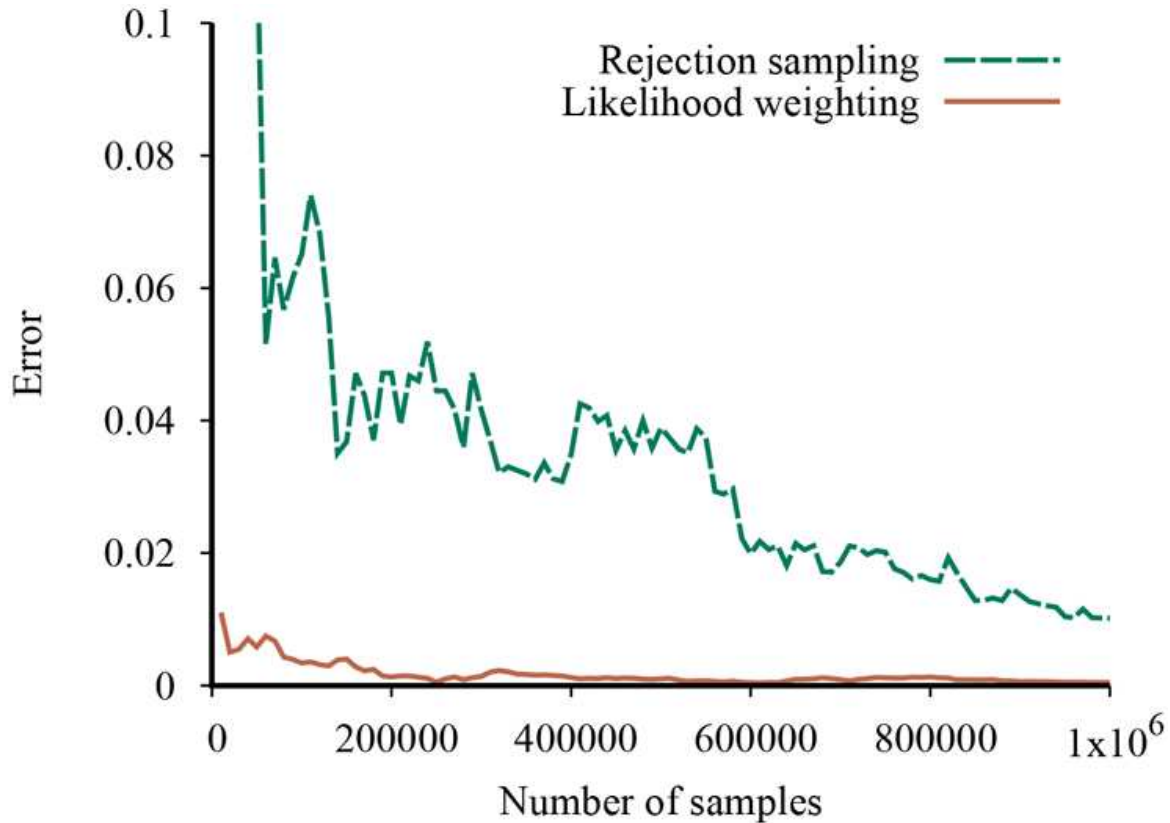
Performance of rejection sampling and likelihood weighting on the insurance network. The x-axis shows the number of samples generated and the y-axis shows the maximum absolute error in any of the probability values for a query on PropertyCost .
