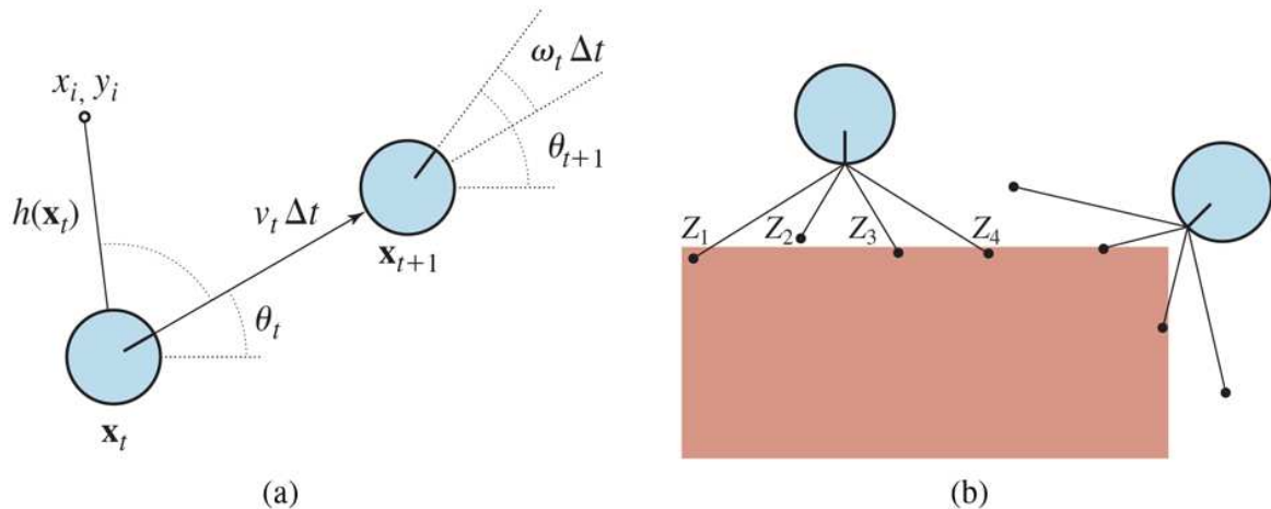
(a) A simplified kinematic model of a mobile robot. The robot is shown as a circle with an interior radius line marking the forward direction. The state \mathbf{x}_t consists of the (x_t, y_t) position (shown implicitly) and the orientation \theta_t . The new state \mathbf{x}_{t+1} is obtained by an update in position of v_t \Delta t and in orientation of \omega_t \Delta t . Also shown is a landmark at (x_i, y_i) observed at time t . (b) The range-scan sensor model. Two possible robot poses are shown for a given range scan (z_1, z_2, z_3, z_4) . It is much more likely that the pose on the left generated the range scan than the pose on the right.
