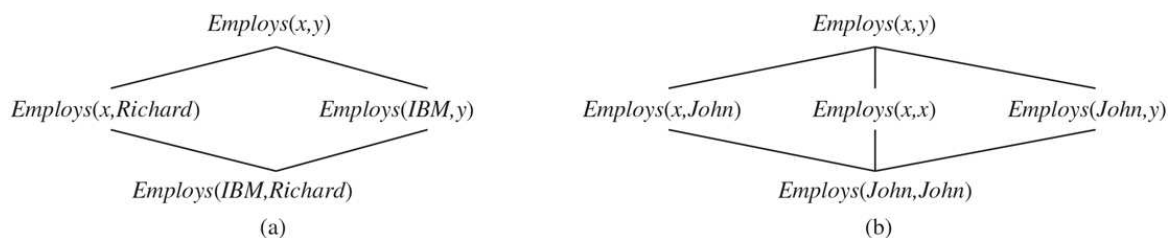
(a) The subsumption lattice whose lowest node is Employs(IBM, Richard) . (b) The subsumption lattice for the sentence Employs(John, John) .
